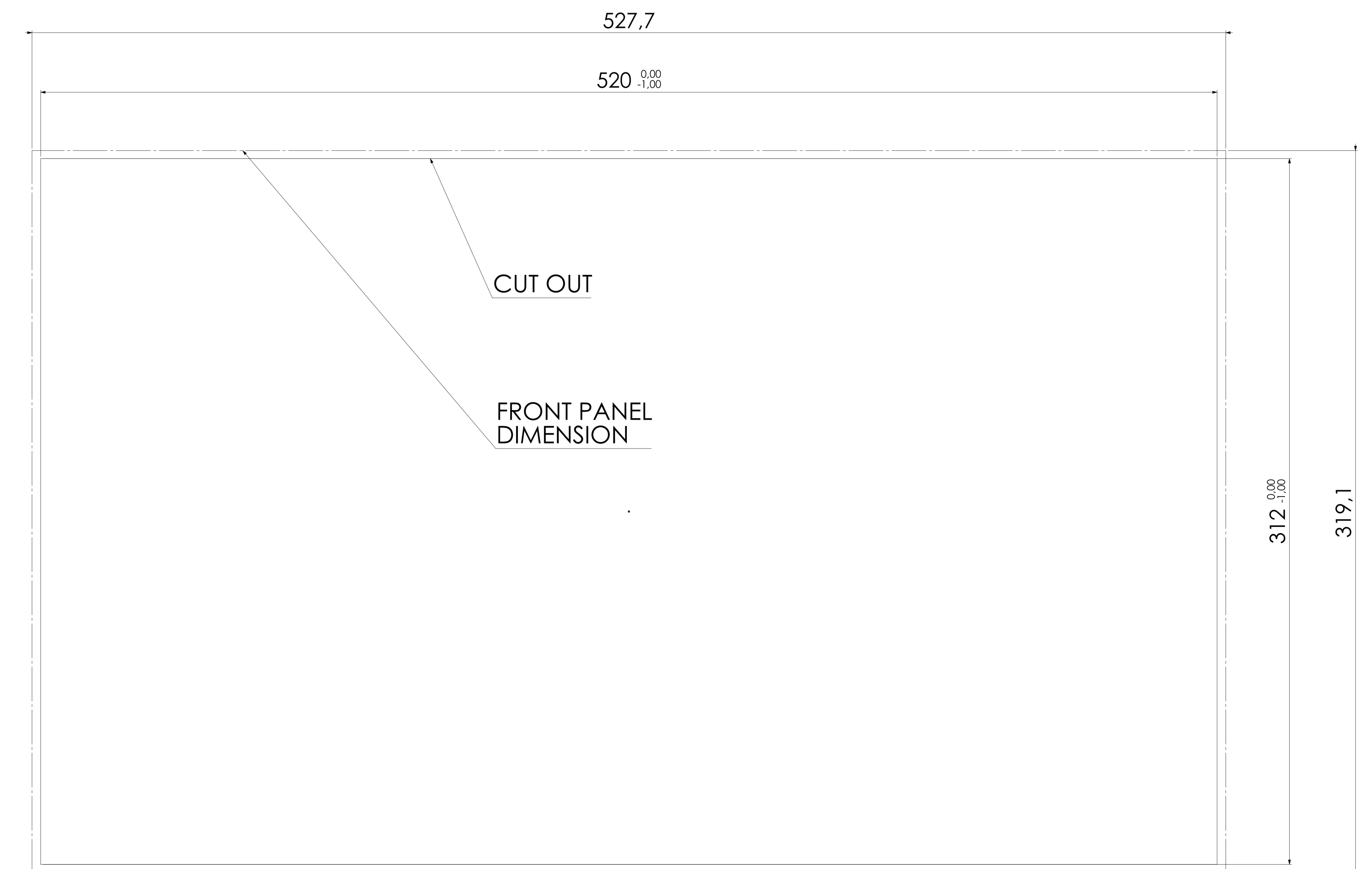
VersaView 6300P (Fanless) 6300P-215ECPMFDNA 21.5 Inch Display dimensions are in mm
