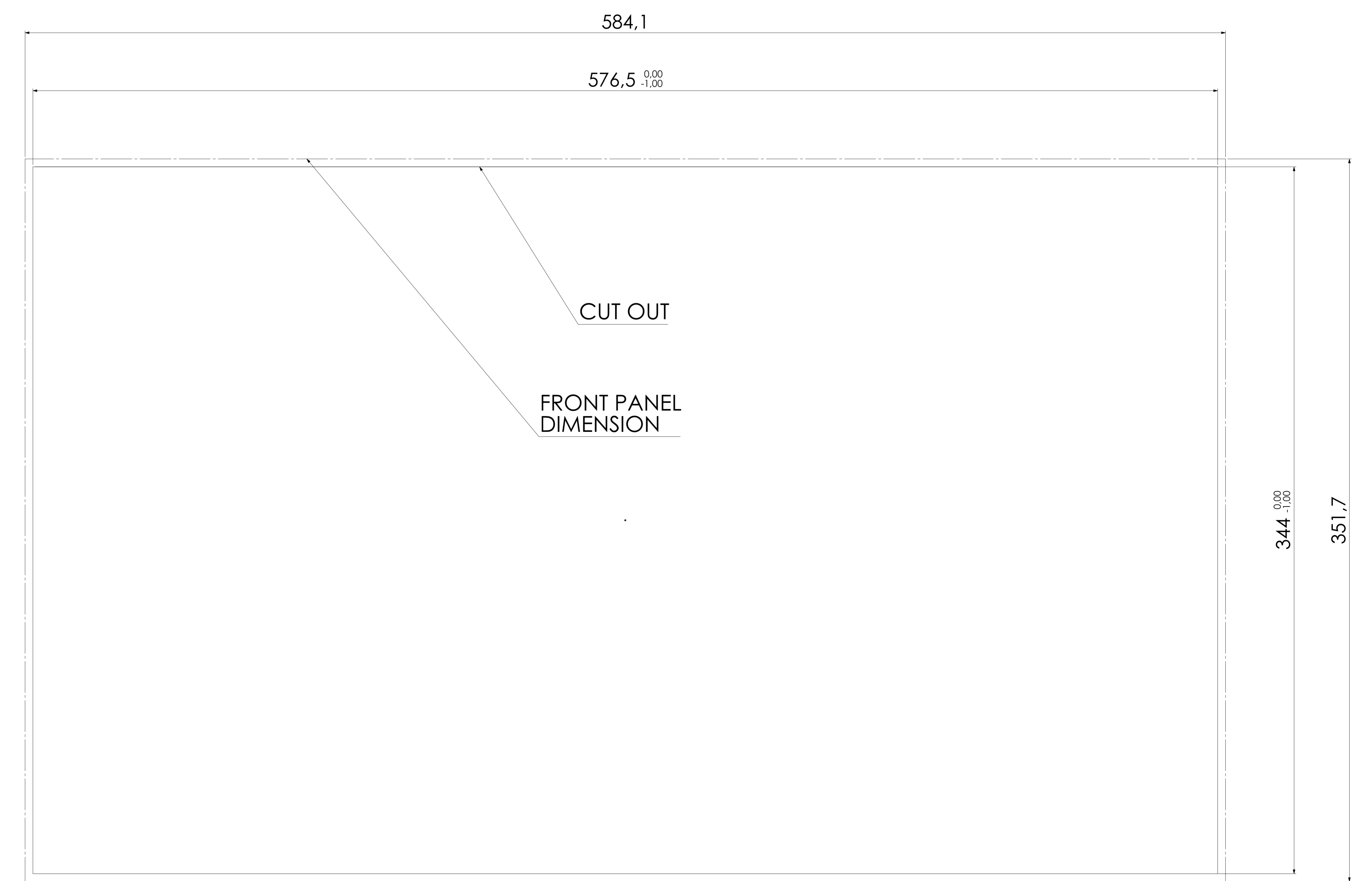
VersaView 6300P (Fanless) 6300P-240ECPMFDA 24.0 Inch Display dimensions are in mm
